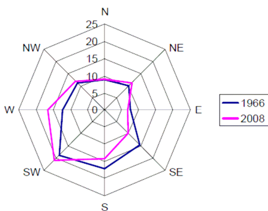
Fig. 8. Distribution of ground-boundary wind direction at regional level according to the Väike-Maarja meteorological station located close to the Lahemaa monitoring site (Jaagus and Kull, 2011).
