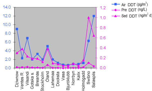
Fig. 4. Summary of DDT concentrations in the air and calculated depositions (based on Agrell et al., 2001). Pre – precipitation, Sed – deposition sedimentation.
