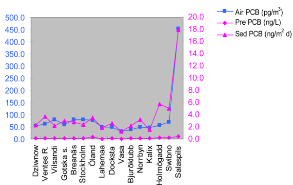
Fig. 2. Summary PCB concentrations in the air and calculated depositions (based on Agrell et al., 2001). Pre – precipitation, Sed – deposition sedimentation.
