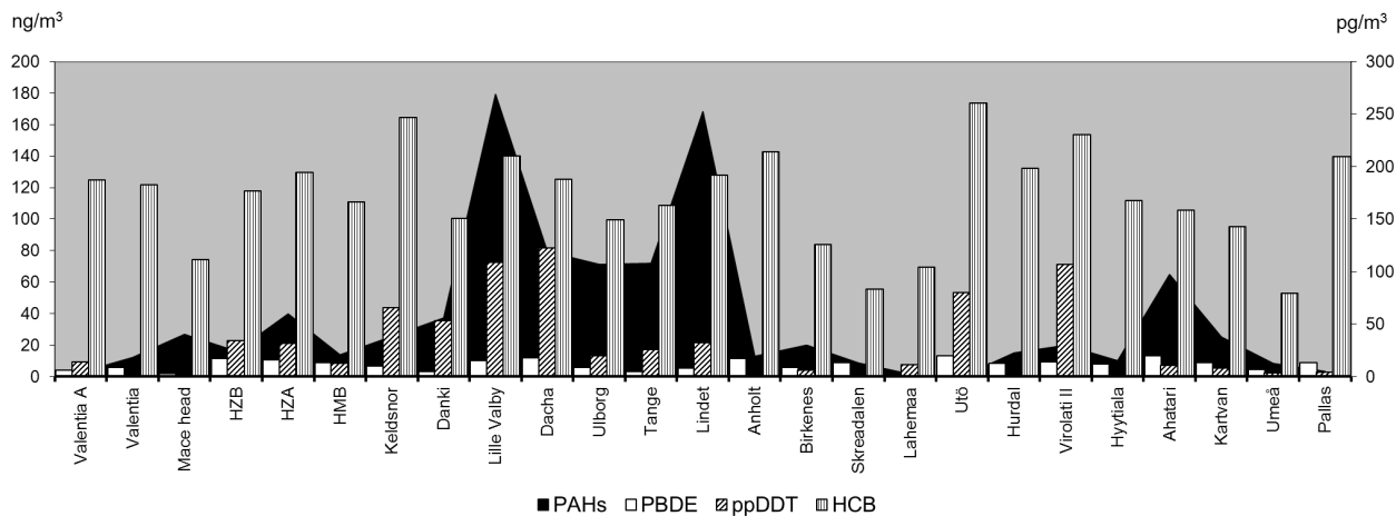
Fig. 5. Concentrations of POPs (pg/m 3 ) and PAHs (ng/m 3 ) in the air at the Lahemaa station and concentration ranges for other sites (Gioia et al., 2007; A. Sweetman, personal information). HZA, HZB, HMB – replicate samplers at the Hazelrigg and High Muffles sites.
