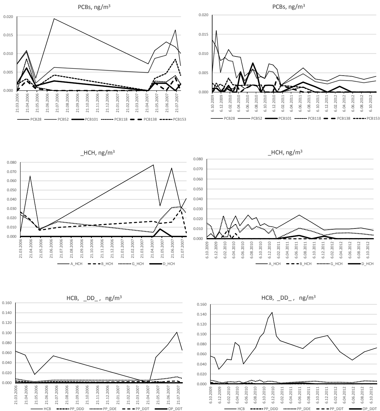
Fig. 10. Seasonal pattern of analysed POPs in the air at the Lahemaa station in 2006–2007 and 2009–2012 (RECETOX, GENASIS database system www.genasis.cz ).
