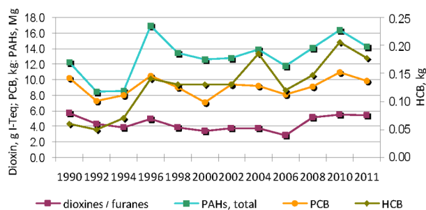
Fig. 6. Emissions of POPs and PAH in the period 1990–2011 (Kohv et al., 2013).
