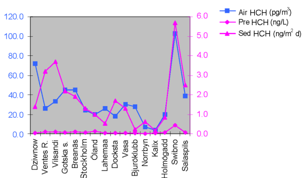
Fig. 3. Summary HCH concentrations in the air and calculated depositions (based on Agrell et al., 2001). Pre – precipitation, Sed – deposition sedimentation.
