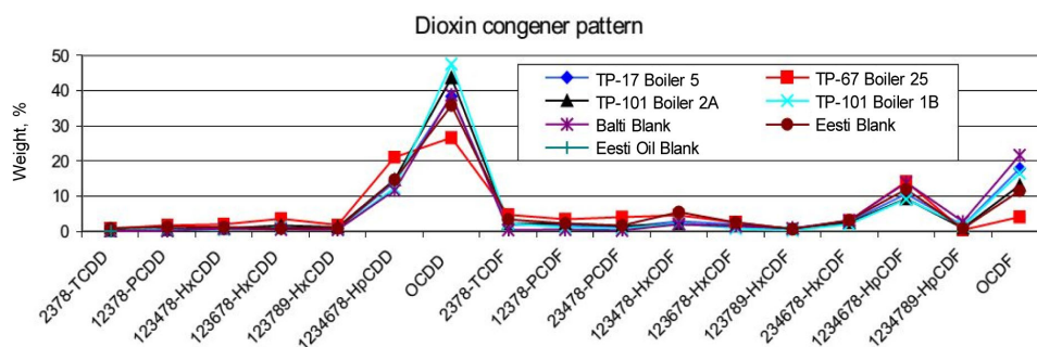
Fig. 7. Dioxin congener pattern for all emission samples and blanks (Schleicher et al., 2004b).
